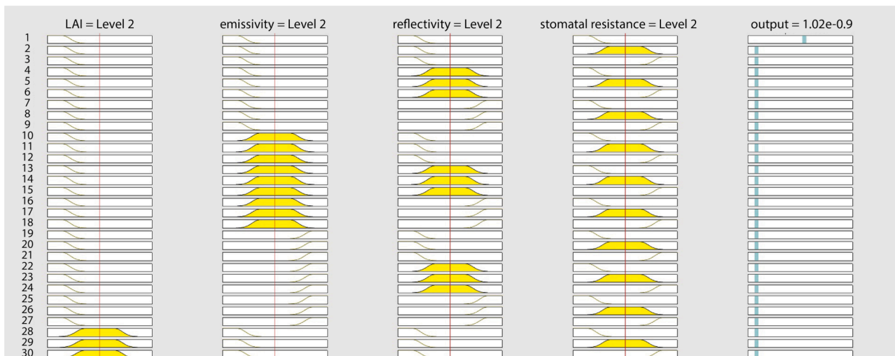
Fig. 10. ANFIS rule structure for Et as a target of this study.
