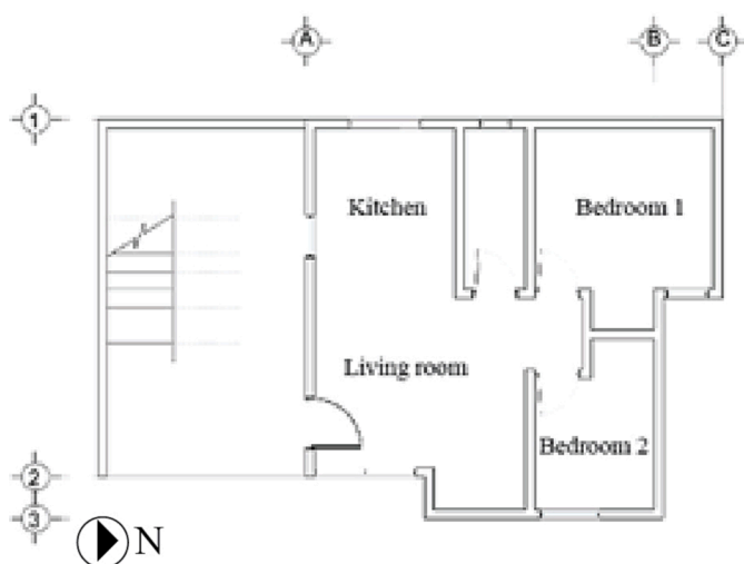
Fig. 6. Typical plan and perspective view of the case study building.
