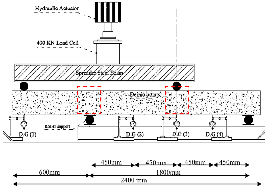
30 31 32 33 34 35 36 Figure 4 Test setup 37 38 39 40 41
