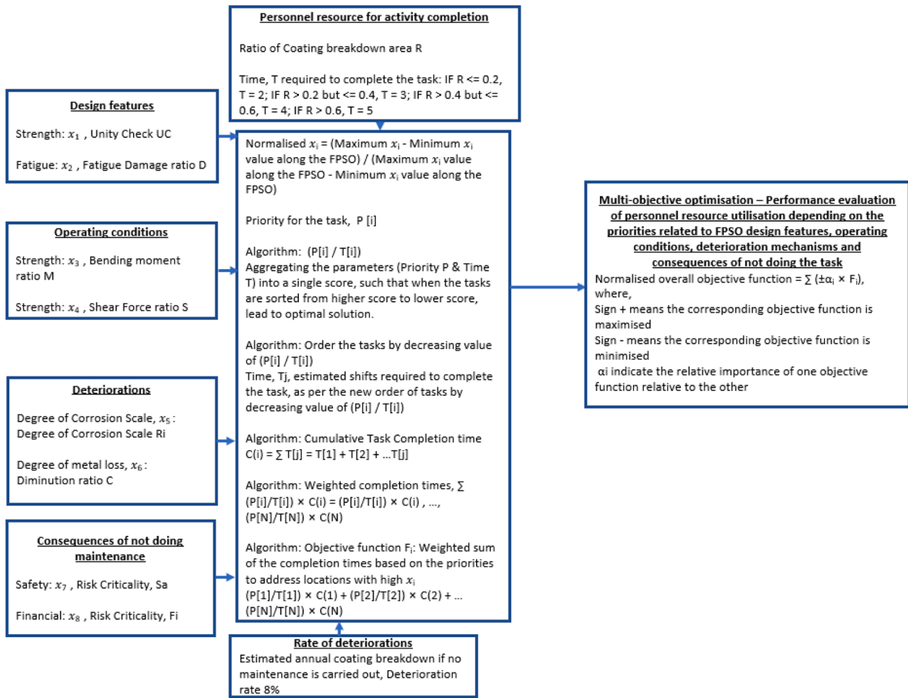
Fig. 16. FPSO system overall multi-objective optimisation problem.
