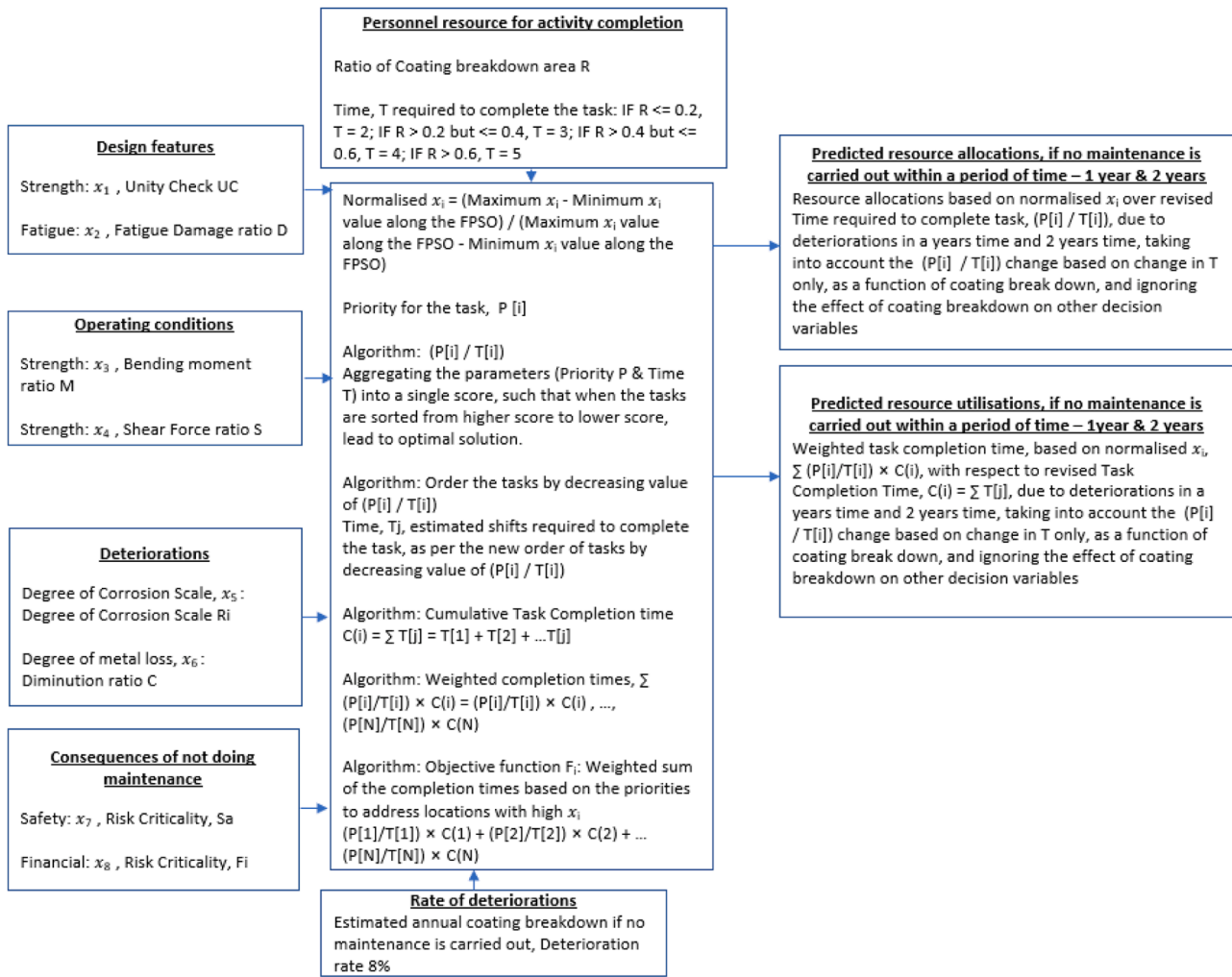
Fig. 11. FPSO system evaluation on maintenance priorities and productivities over a period of time.
