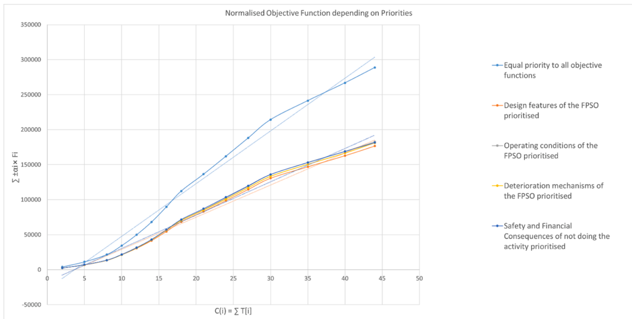
Fig. 17. Overall objective optimisation depending on Priorities.
