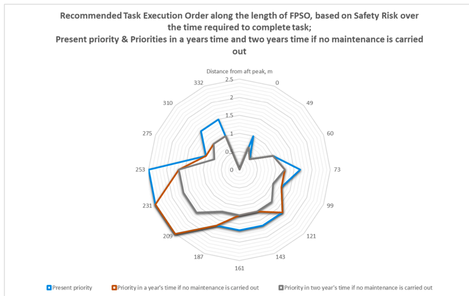
Fig. 12. Changes in resource allocations if no maintenance is carried out, based on Consequences of not doing tasks–normalised Safety Risk over time required to complete task.
