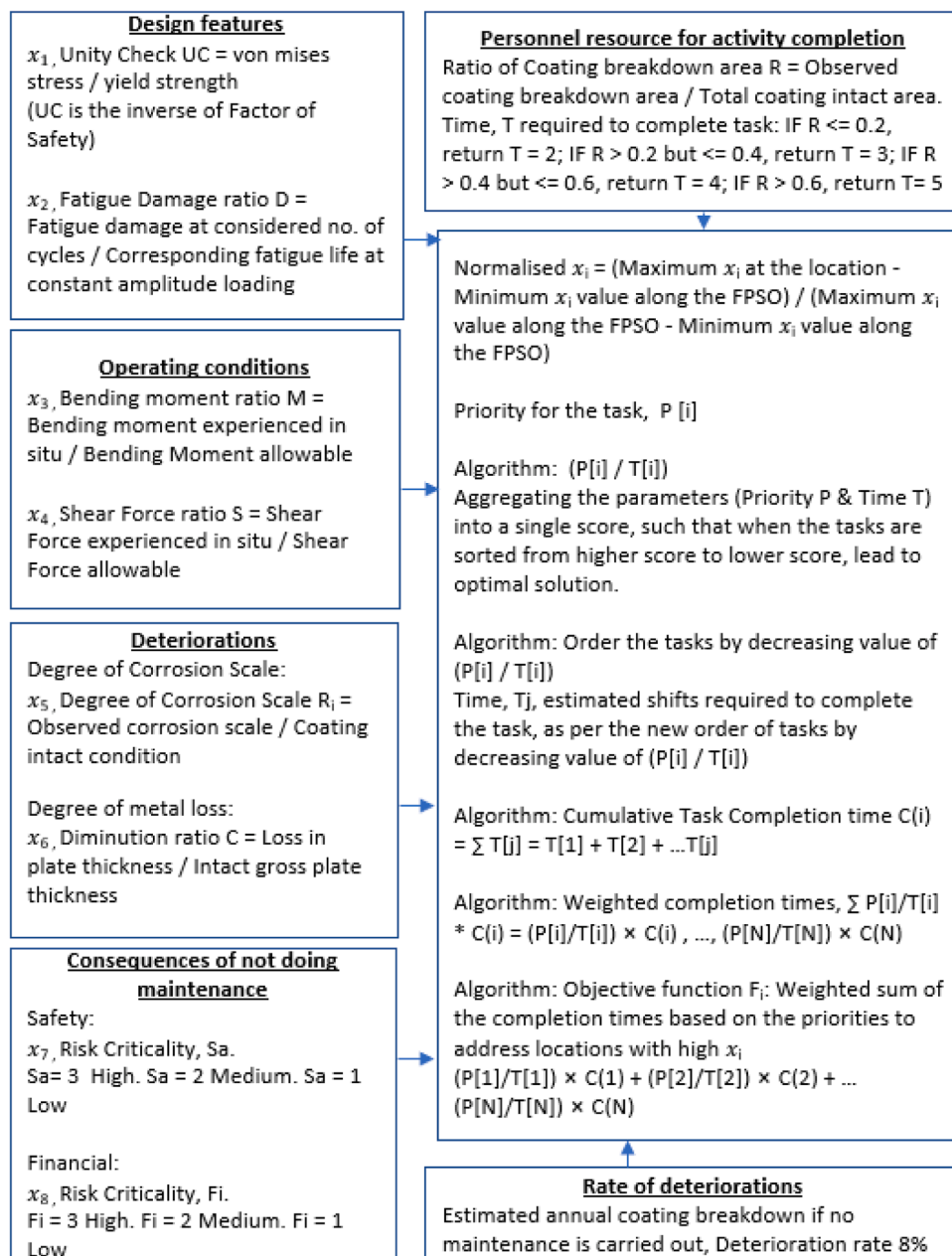
Fig. 5. Methodology of FPSO main deck maintenance planning problem.
