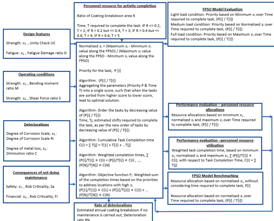
Fig. 6. FPSO system optimisation problem.
