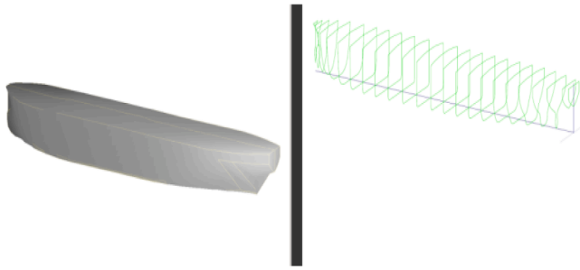
Fig. 1. Profile of the modelled FPSO.
