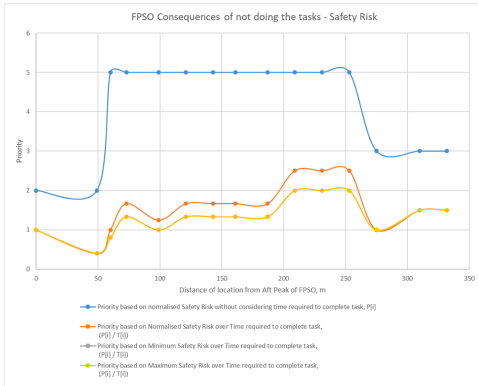
Fig. 7. Resource allocation based on Consequences of not doing the tasks – Safety Risk over Time required to complete task, (P[i] / T[i]) .
