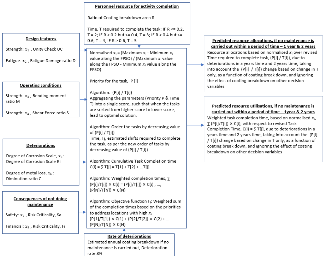
Figure 10: FPSO system evaluation on maintenance priorities and productivities over a period of time
