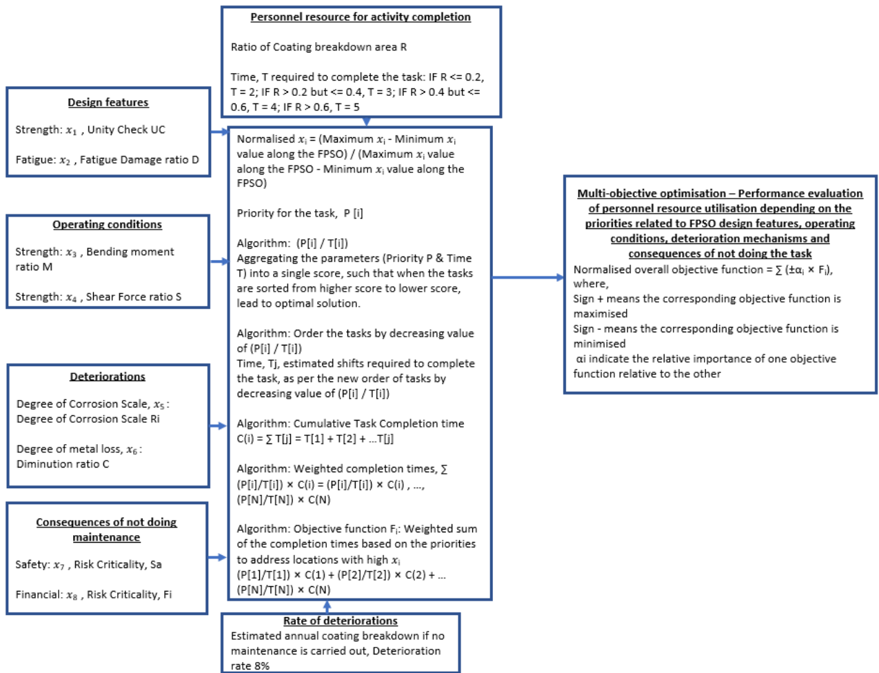
Figure 15: FPSO system overall multi-objective optimisation problem
