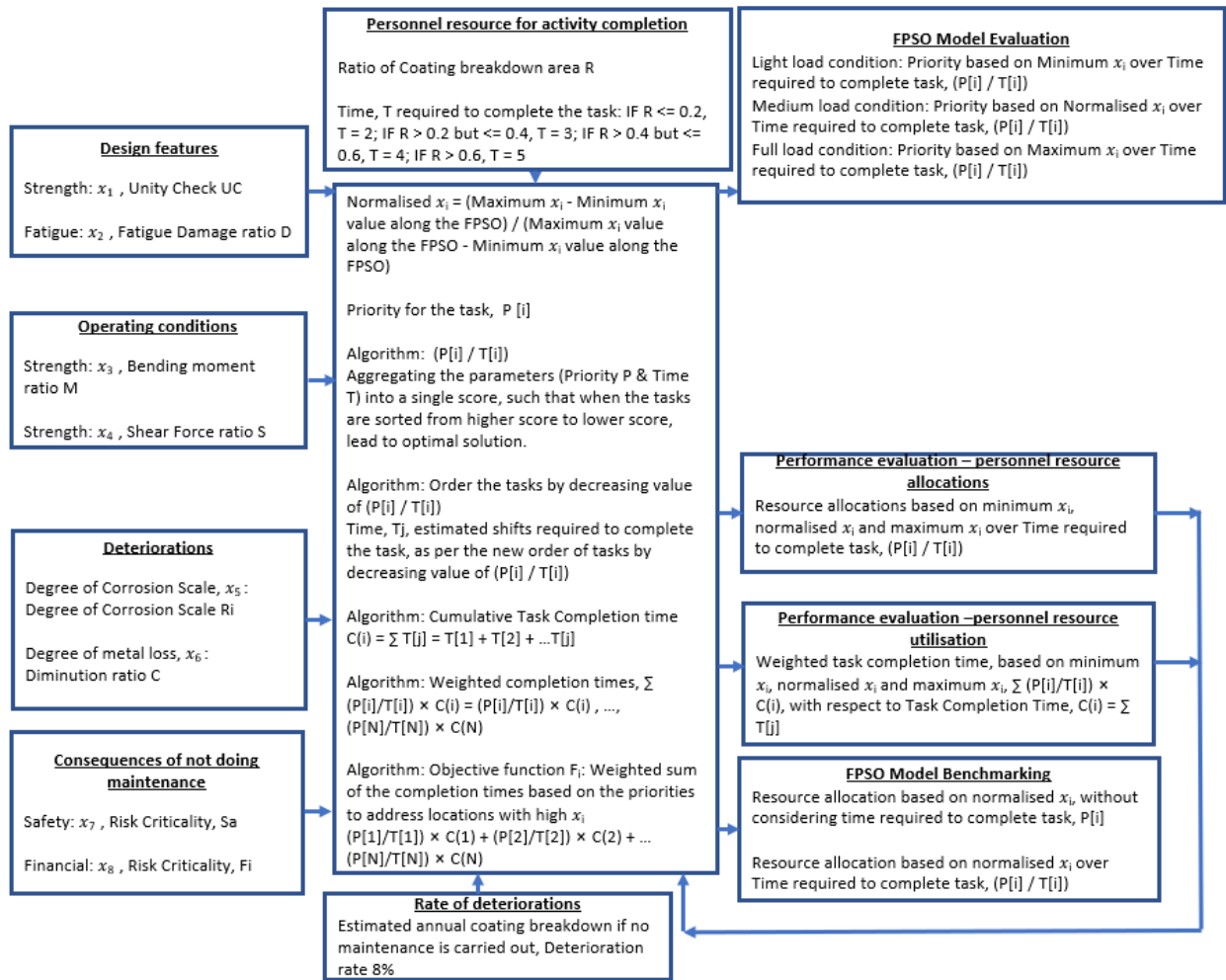
Figure 5: FPSO system optimisation problem
