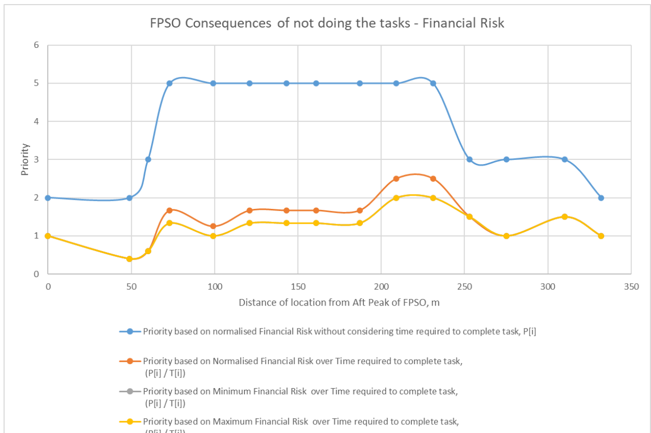
Figure 8: Resource allocation based on Consequences of not doing the tasks – Financial Risk over Time required to complete task, (P[i] / T[i])
