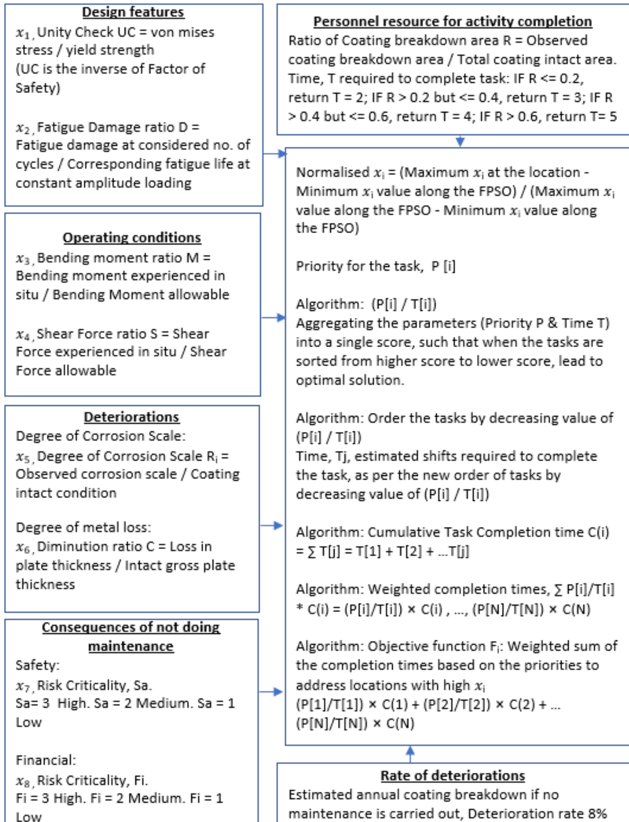
Figure 4: Methodology of FPSO main deck maintenance planning problem
