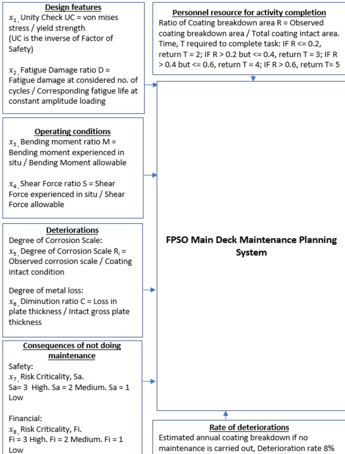
Figure 3: FPSO Main Deck maintenance planning system problem
