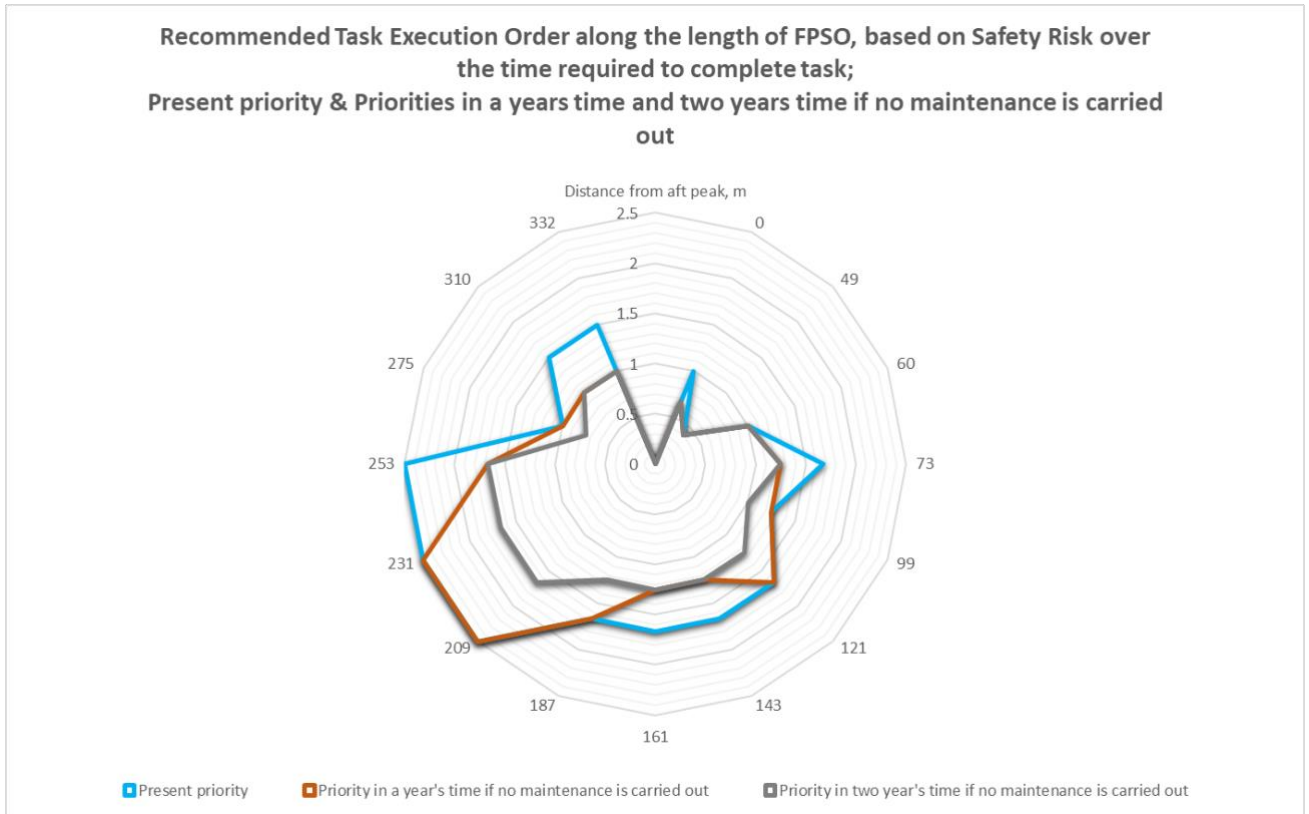
Figure 11: Changes in resource allocations if no maintenance is carried out, based on Consequences of not doing tasks–normalised Safety Risk over time required to complete task
