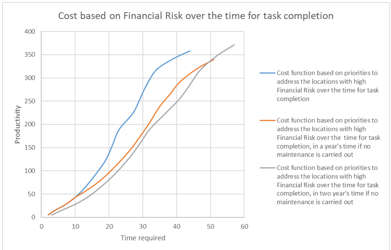
Figure 14: Changes in resource utilisations if no maintenance is carried out, based on Consequences of not doing the tasks – normalised Financial Risk over the time required to complete task
