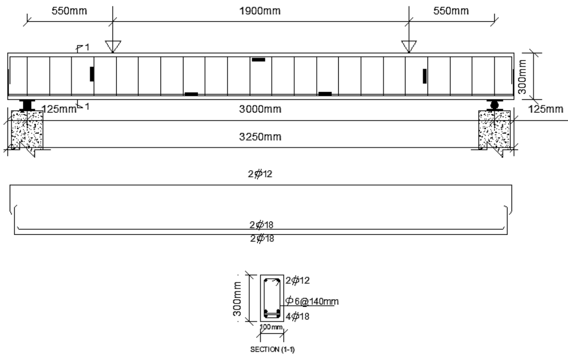
b. Reinforcement details and strain gauges' positions for beams tested in shear
