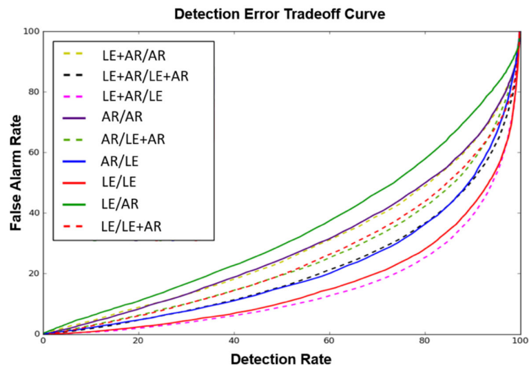
Figure 5. DET Curves for each of the recognition experiments. The first montage indicator refers to the data used for training, while the second one refers to the evaluation set. For example, LE +AR/AR refers to a model trained with LE+AR data and evaluated with AR data.
