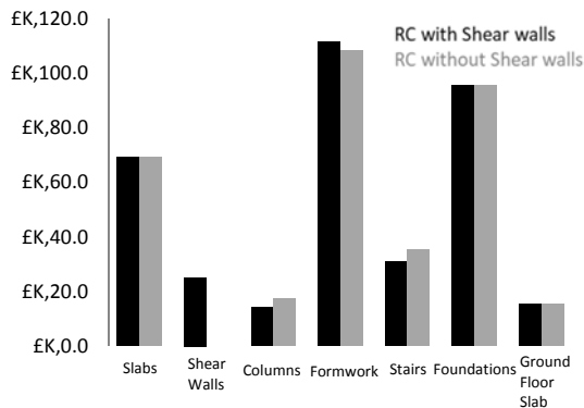
Fig. 8 Comparison of Structural Components cost
