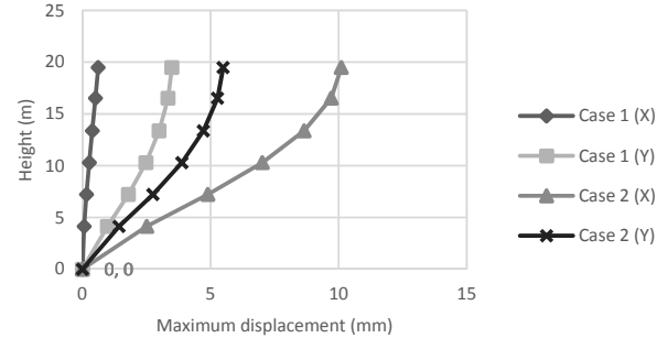
Fig. 5 Comparison of maximum displacement in Case 1&2
