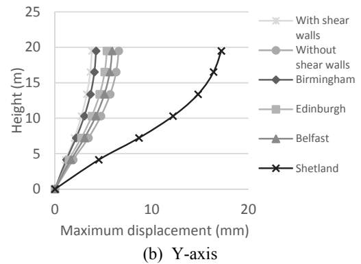
Fig. 9 Comparison of Maximum Displacements in all locations
