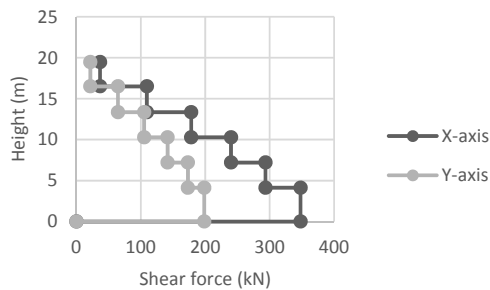
Fig. 7 Shear force comparison case 2 (X & Y axis)
