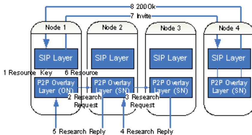
Fig. 1: The architecture of a P2P SIP network
