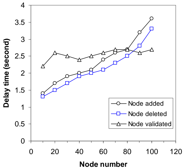
Fig. 8: The delay time of the authentication algorithm
