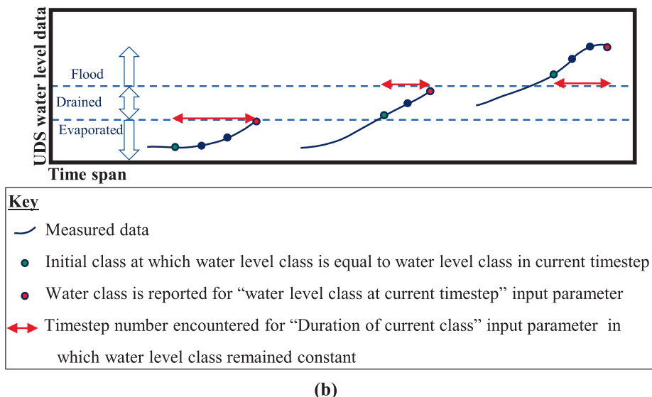
Fig. 2. Structure of proposed new features for (a) rule-based BPNN model for rainfall RP prediction, (b) proposed water class data featuring.
