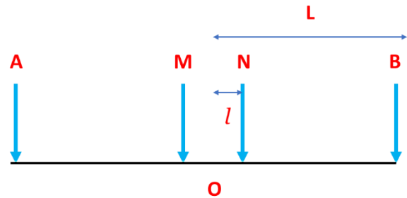
Figure 1. Schematic representation of the Schlumberger array configuration. Points A and B represent the current electrodes, while M and N denote the potential electrodes. The distances 2L and 2l correspond to the separation between the current electrodes and the potential electrodes, respectively, with O representing the midpoint of the array
