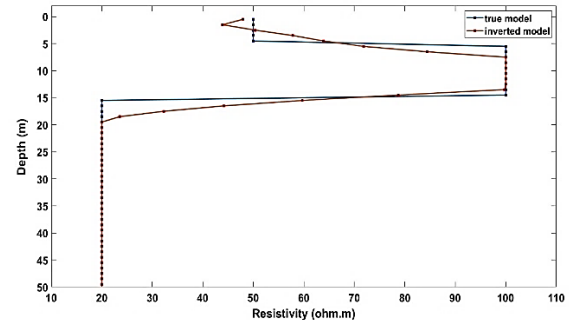
Figure 4. The comparison of the true and inverted model from 5% noisy data.
