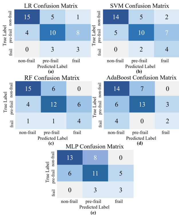
Fig. 3 Confusion matrices for the testing set of ML algorithms: a Logistic Regression (LR), b Support Vector Machine (SVM), c Random Forest (RF), d AdaBoost, e Multi-Layer Perceptron (MLP)
