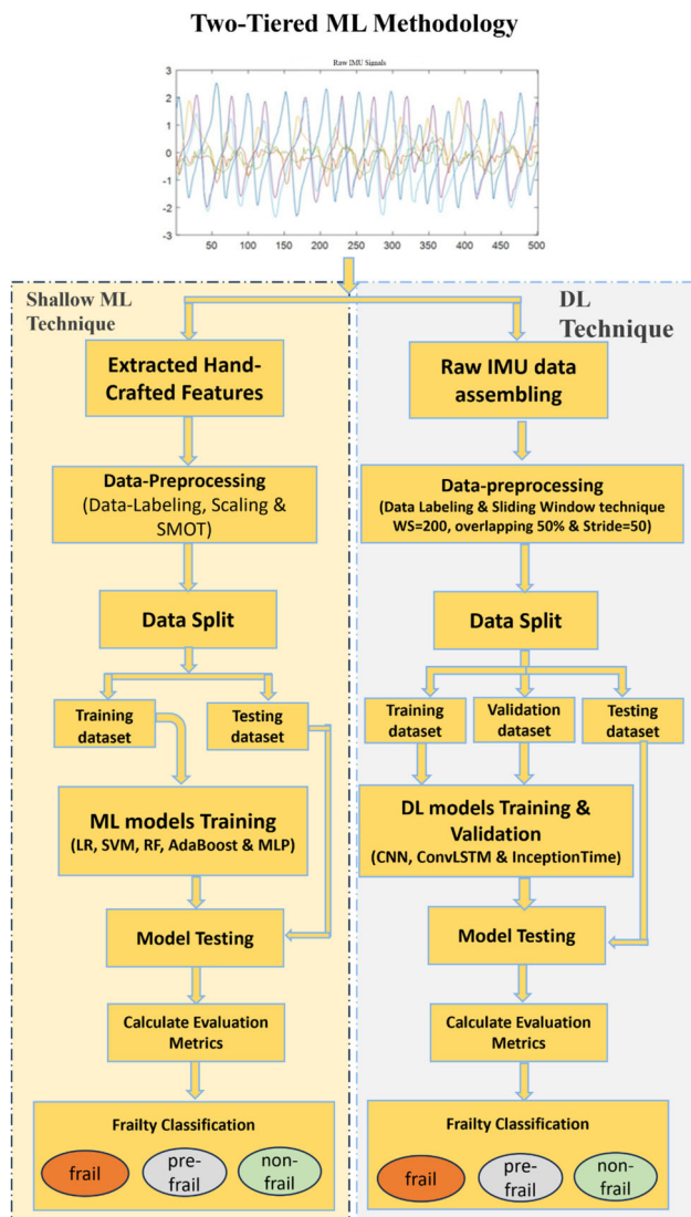
Fig. 1 Two-Tiered research methodology that used both shallow ML techniques and DL techniques for frailty classification
