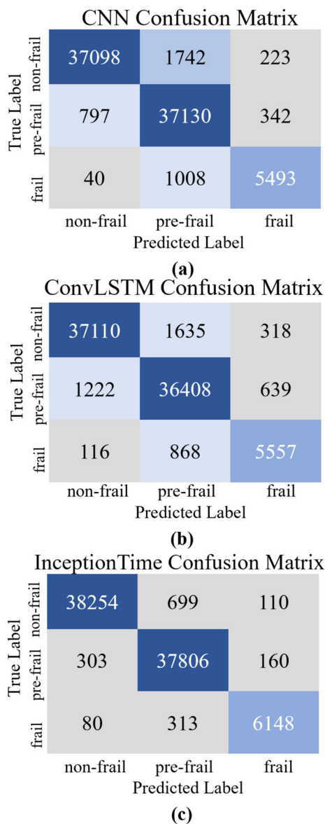
Fig. 5 Confusion matrices for the testing set of DL algorithms: a CNN, b ConvLSTM and c InceptionTime
