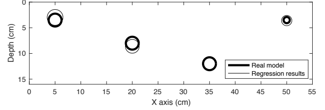
Fig. 6. The actual and the predicted rebar diameter and location using the proposed regression scheme. The inputs are real compressed A-scans collected with the antenna directly above the rebar on the surface of the (well-cured) concrete slab.
