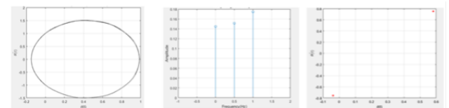
Fig. 3: Phase portrait, frequency-domain plot and Poincaré map when \Omega = 21.042 rad/sec.
