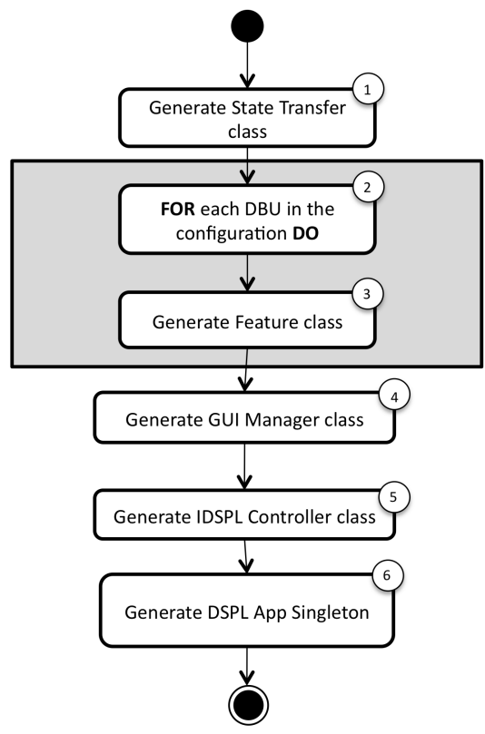
Figure 7.3: Generated Support Classes
