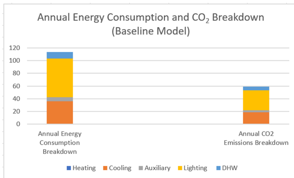
Figure 16. Annual Energy Consumption and CO 2 Breakdown.
