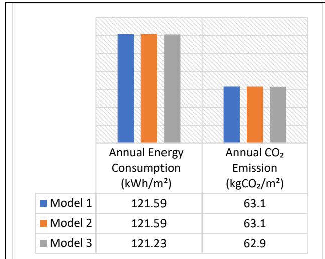
Figure 32: Model P1, P2 and P3 - Operational Energy/Carbon emissions under High 90 th scenario.
