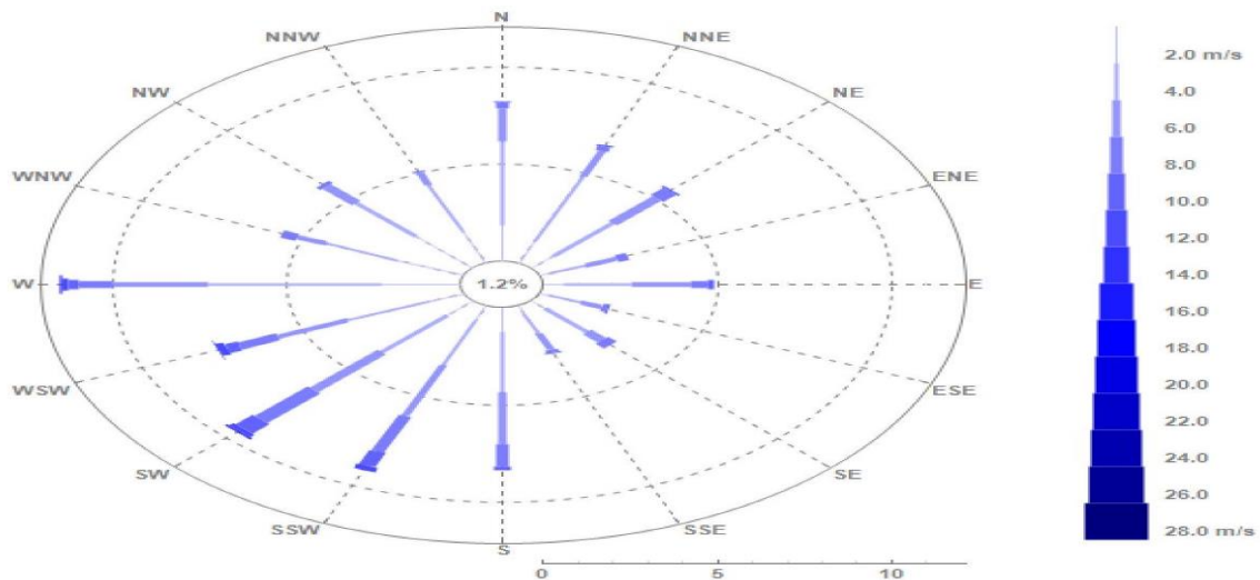
Figure 37a. London test reference year annual wind rose.
