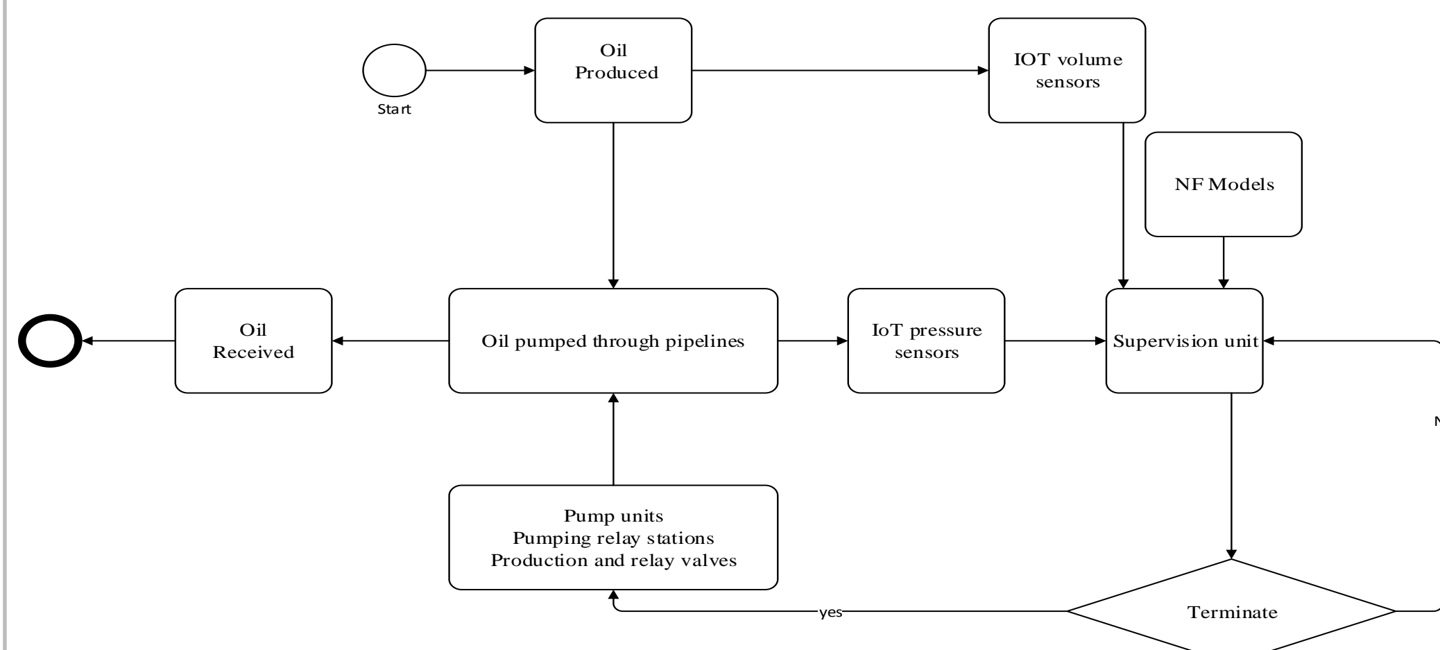
Fig. 1: Oil Pipeline Supervision System Flowchart
