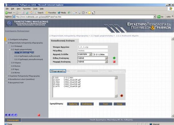
Fig. 1: Authoring environment
