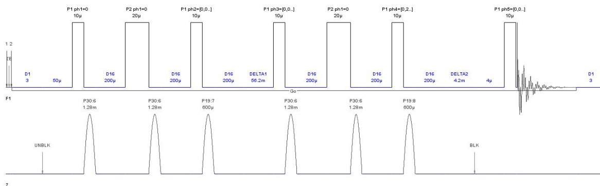
Figure S1: Pulse sequence ledbpgp2s used in DOSY experiments
