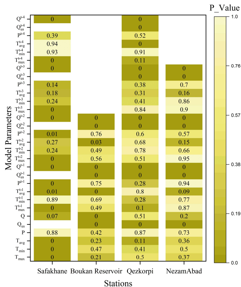
Figure 7. The results of one-way ANOVA sensitive analysis for various input parameters in the RNN network.
