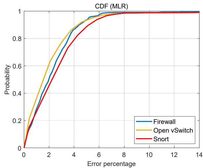
Figure 10. CDF of percentage prediction errors of MLR.
