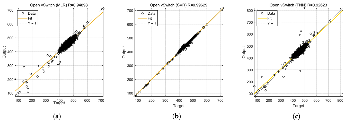
Figure 8. Open vSwitch regression plot: (a) MLR; (b) SVR; and (c) FNN.
