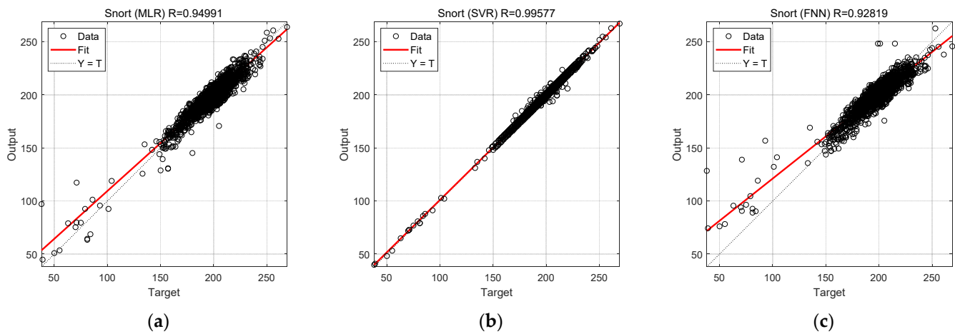
Figure 9. Snort regression plot: (a) MLR; (b) SVR; and (c) FNN.
