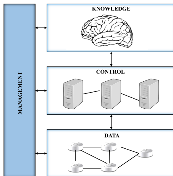
Figure 1. SDN-with-Knowledge plane.
