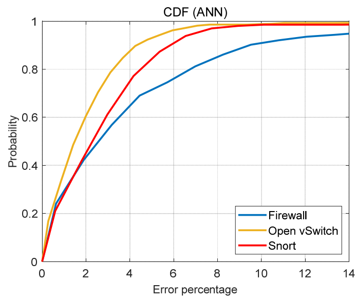
Figure 12. CDF of percentage prediction errors of FNN.
