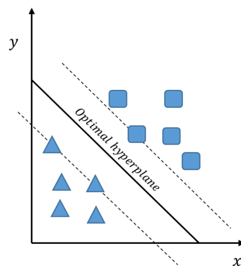
Figure 4. SVM optimal hyperplane.
