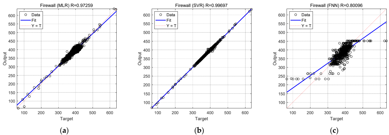
Figure 7. Firewall regression plot: (a) MLR; (b) SVR; and (c) FNN.
