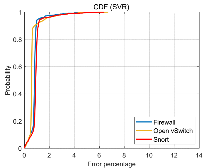
Figure 11. CDF of percentage prediction errors of SVR.
