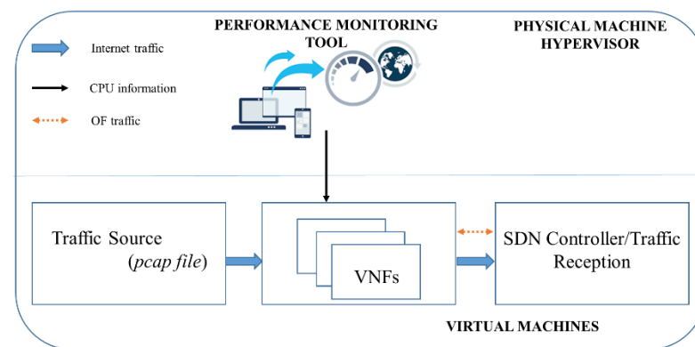
Figure 6. Configuration setup for collecting the data set.
