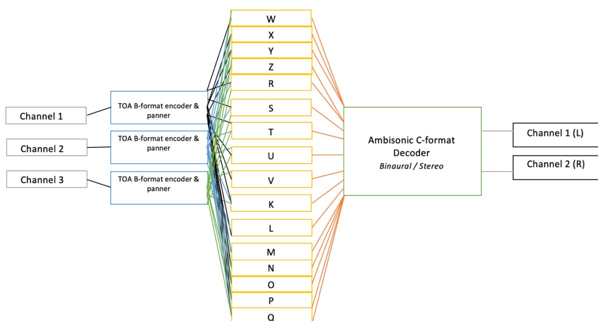
Figure 36: An example of the TOA O3A upmix/decode flow for 3 of the 14 channels. 51
