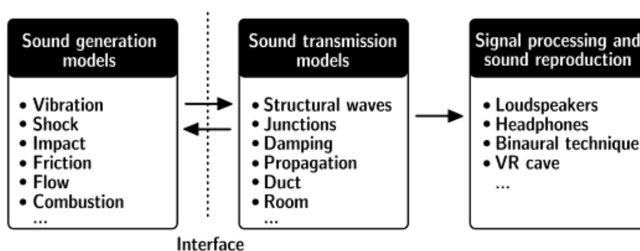
Figure 13: Principles of auralisation (Vorländer, 2008, pg.104)
