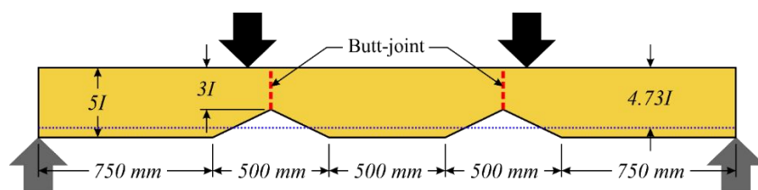
Fig. 13 Simplified beam for deflection analysis
