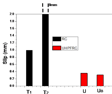
Figure 12. Maximum interface slip results
