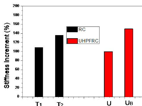
Figure 10. Stiffness increment results
