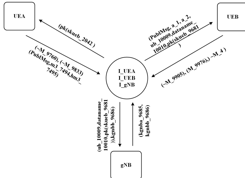
Figure 7. DDSec protocol attack trace.
