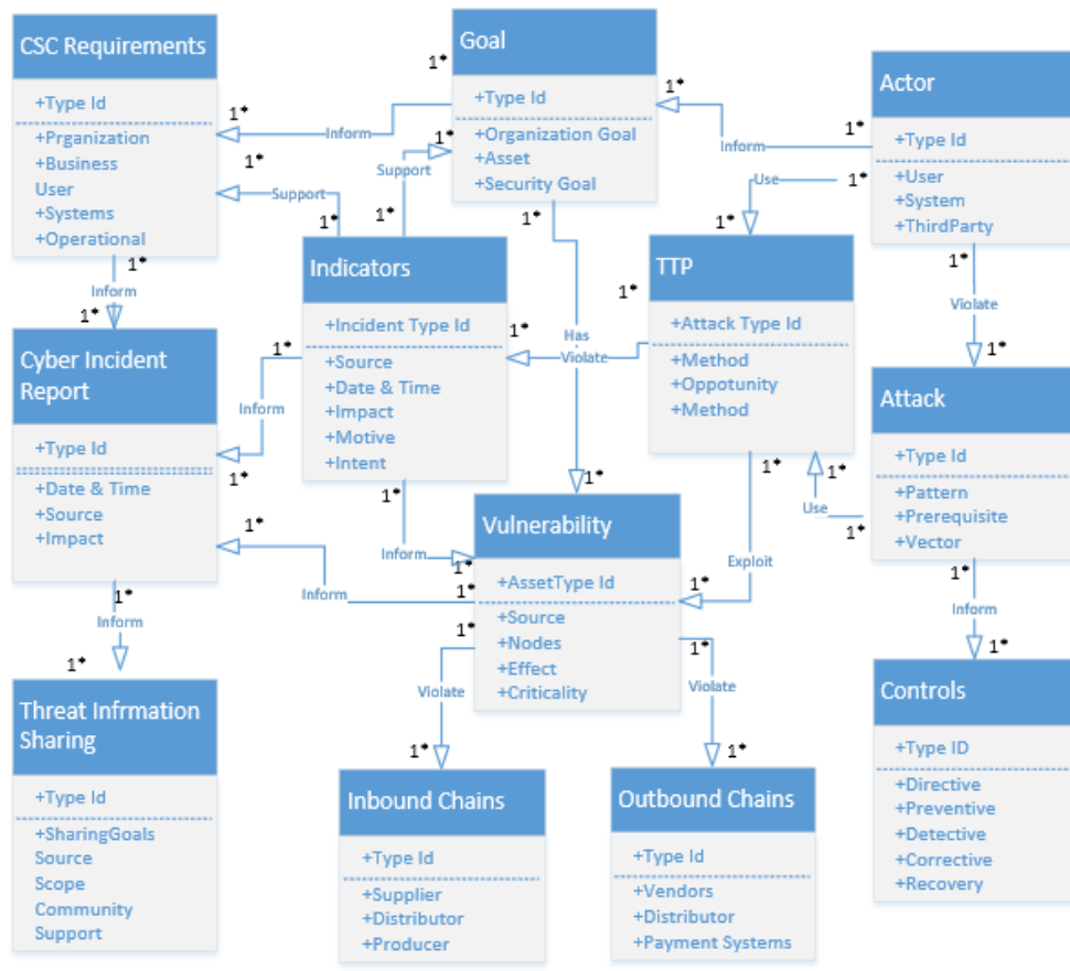
Figure 1: Meta-Model
