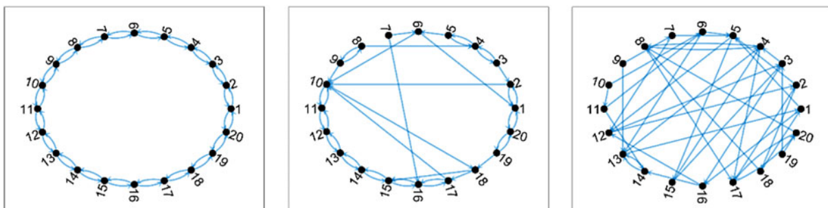
FIG. 11. Example of the creation of a small-world network.
