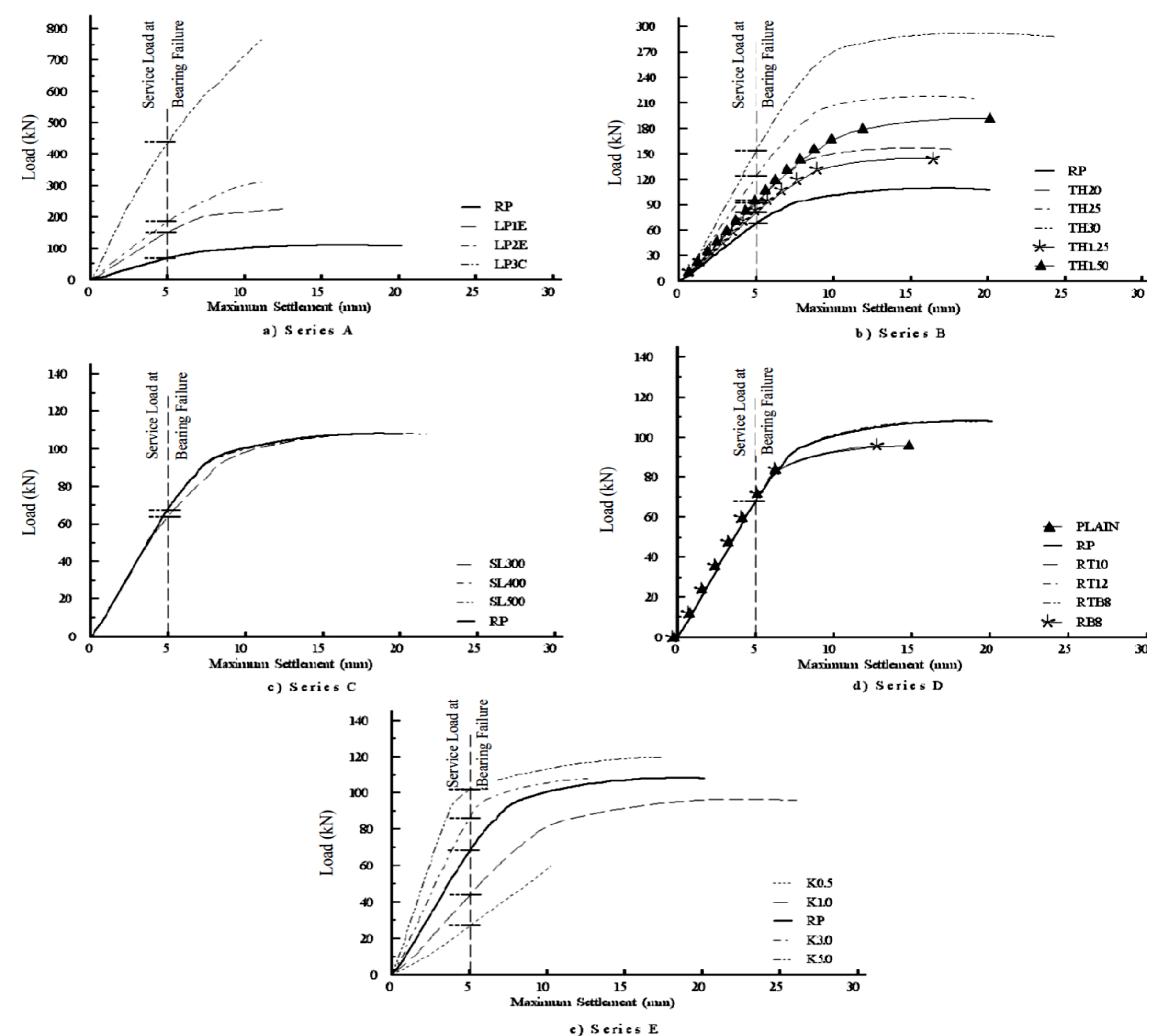
Figure 4 Load-settlement response of the slab panels
