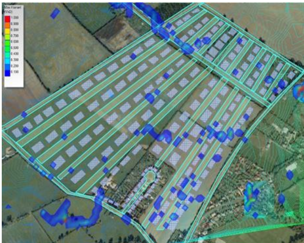
Figure 49 Max Hazard (VxD) after completion of building development
