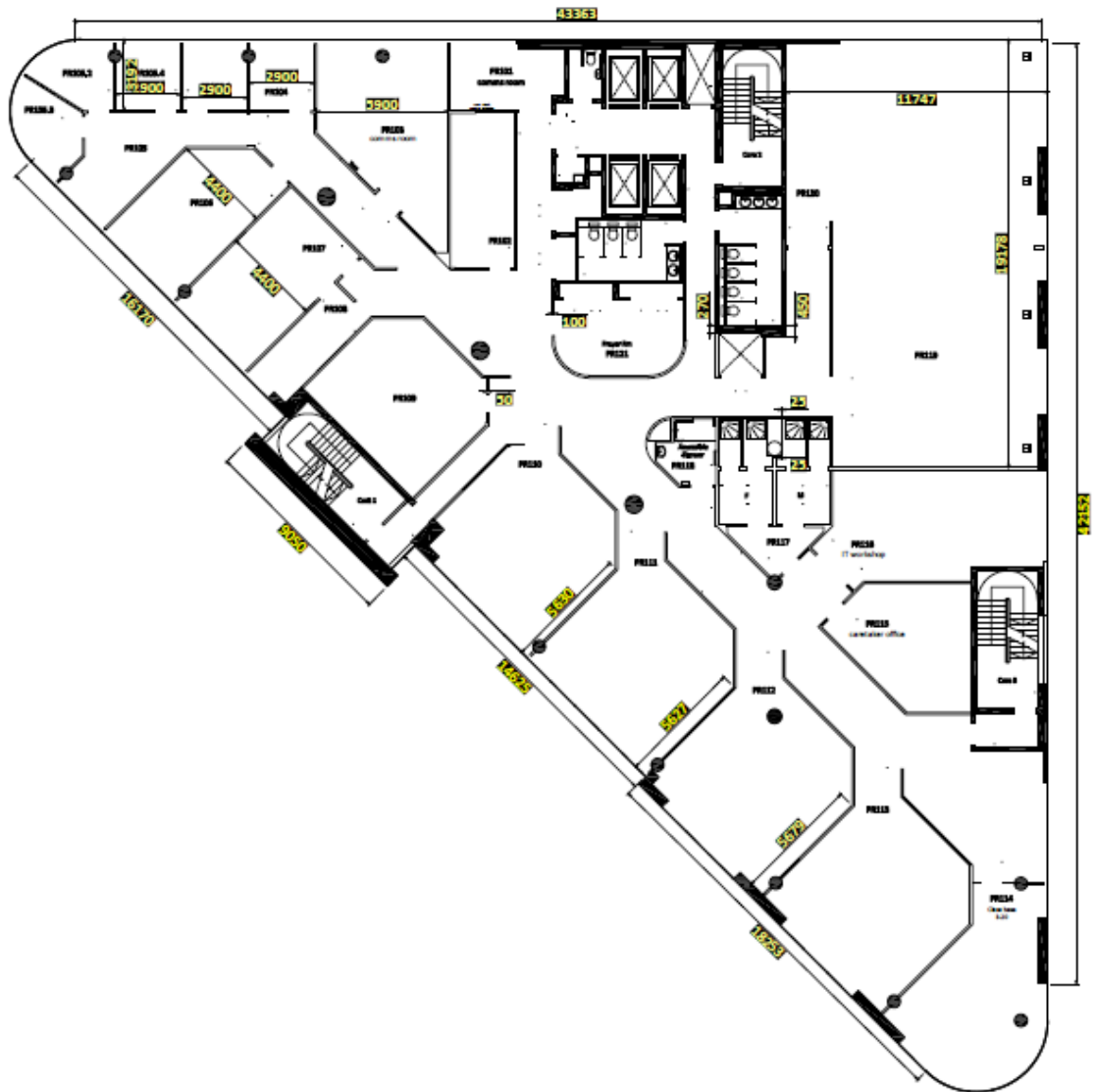
Figure 9 Plan of the first floor of the Paragon building
