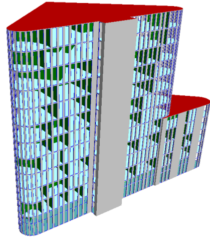
Figure 23 70% Window-to-wall ratio
