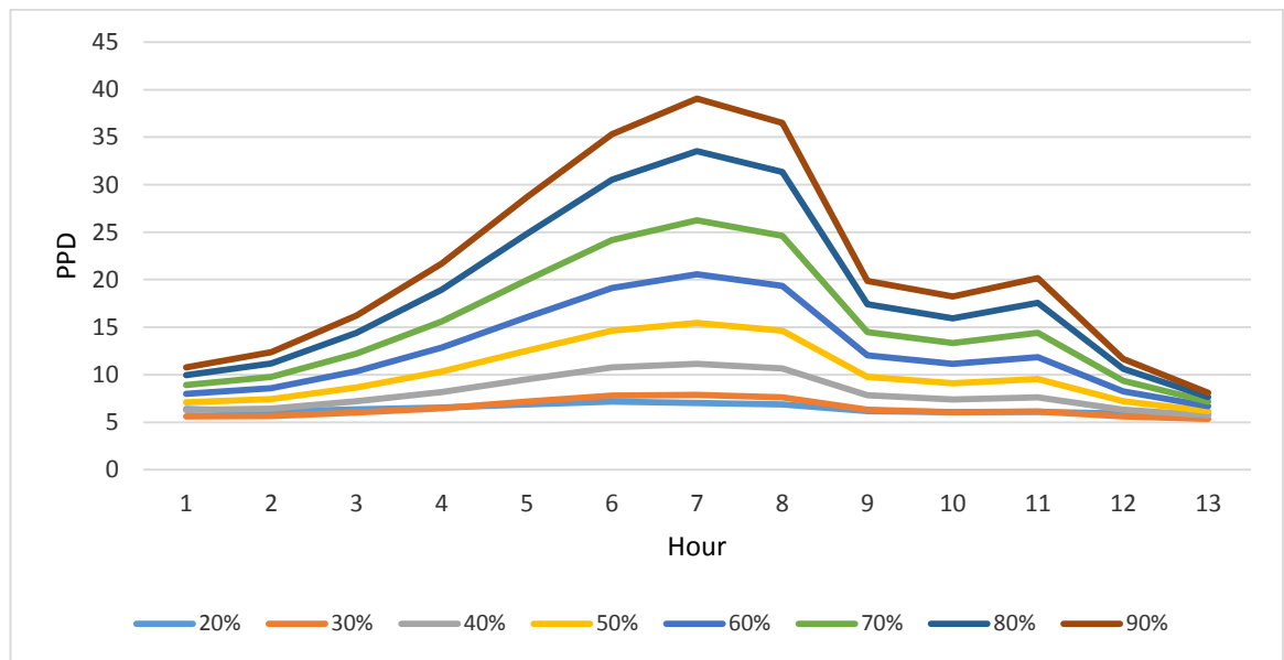
Figure 28 PPD under current weather conditions
