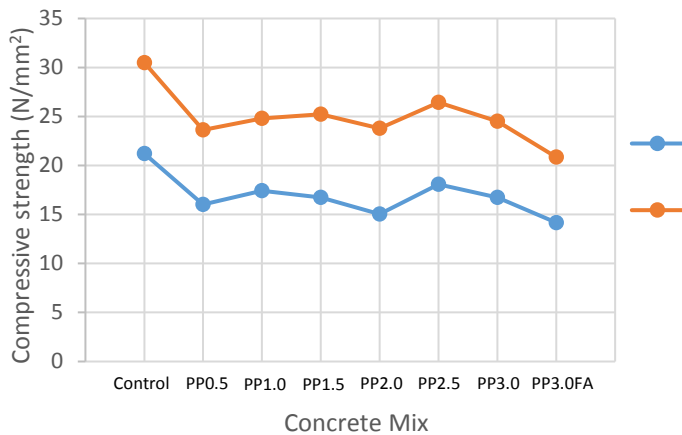
Fig. 8 Compressive Strength Results of All Concrete Mixes at 7- and 28-Days Curing
