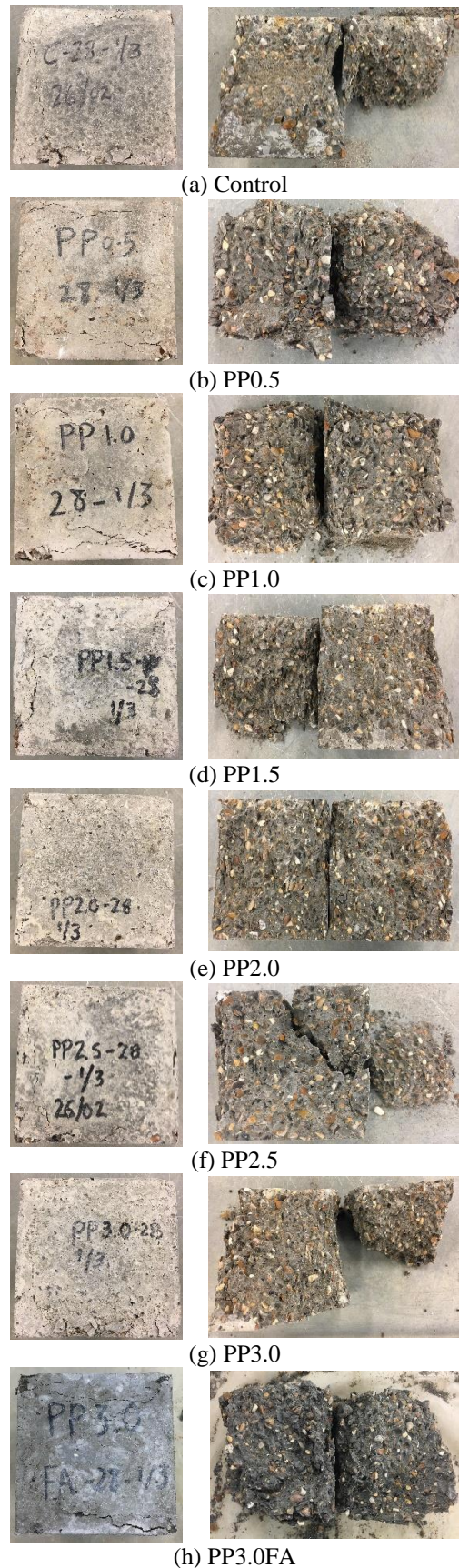
Fig. 9 Breaking of Concrete Cubes – Shown Typically Per Mix at 28-Days Curing
