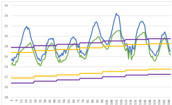
Fig. 4. Comparison of operative temperatures (Bedroom 3)
