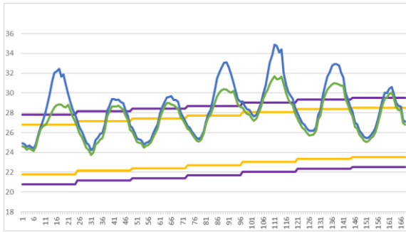
Fig. 3. Comparison of operative temperatures (Bedroom 2)
