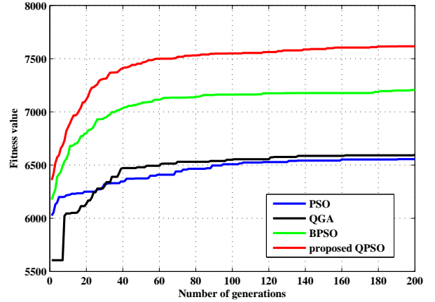
Fig. 4. Number of generations vs. fitness value
