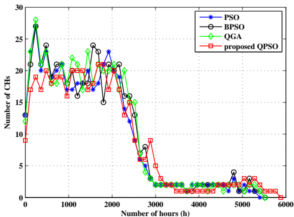
Fig. 7. Number of hours vs. number of CHs
