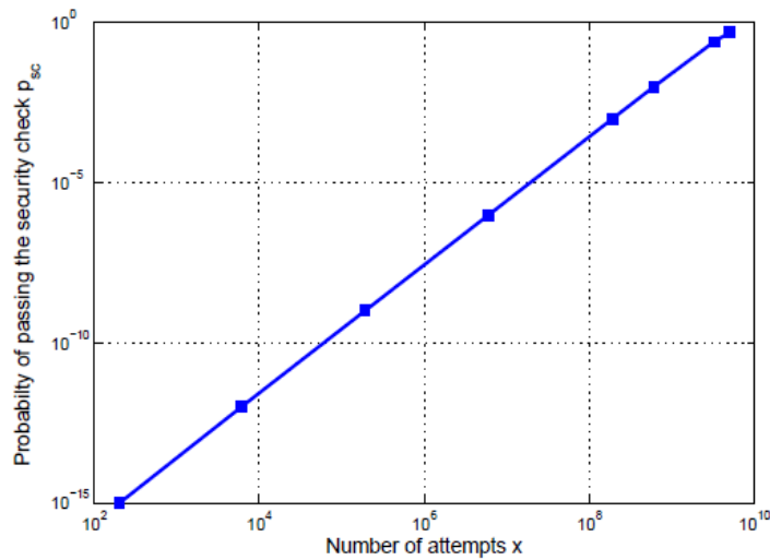
Figure.5. The expected number of attempts required to find a collision in 64-bit long hash for different probability p_{sc} .
